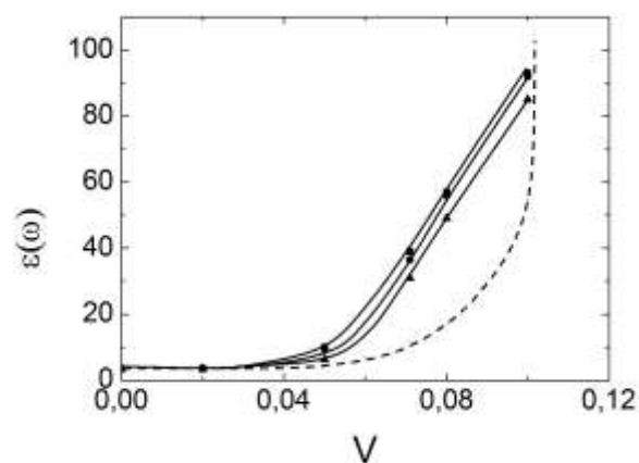
Fig. 5. V-dependences of the permittivity \varepsilon(\omega) for the metal-polymer composites containing nanoscale Ni particles. V-dependences are obtained by measurements at frequency 1000 Hz ( ) and 20 Hz ( ), by extrapolation measured data of the frequency dependences of \varepsilon to the zero frequency ( ), and by calculations in the frame of the percolation theory (the dashed line).
