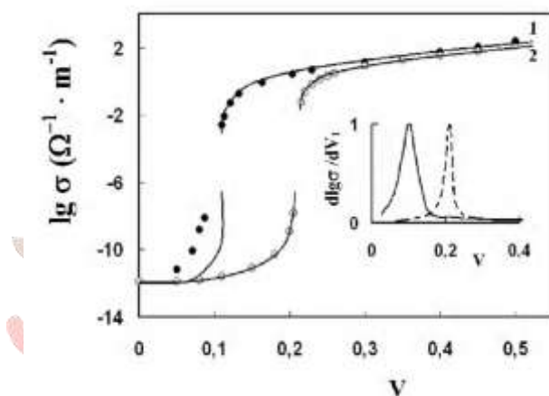
Fig. 2. Comparison of the measured (points) and calculated (solid curves) dependences of the conductivity \sigma on the fractional Ni content V for the metal-polymer composites containing nanoscale Ni particles (full points, curve 1) and micro-dispersed Ni particles (empty points, curve 2). In the insert are shown plots of the dependence of d \lg \sigma / dV on V (the solid line is for the composite containing nanoparticles, the dashed line is for the composite containing micro-dispersed particles).
